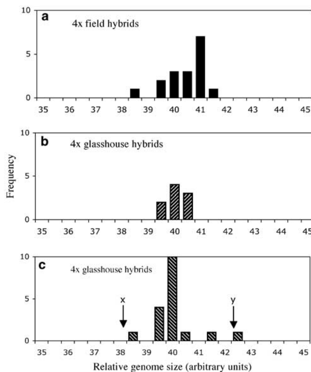
Figure 5 Frequency chart of genome size estimates, expressed as H. pilosella -relative chromosome number, from flow cytometry of (a) hybrid Hieracium from the field, and (b) the progeny of two glasshouse crosses between H. pilosella 4 × mother × H. praealtum 4 × father, and (c) field hybrid 4 × mother × H. praealtum father. Arrows on (c) indicate DNA content estimates that correspond to size classes expected from (x) 3pil,1pra and (y) 1pil,3pra genomes.
